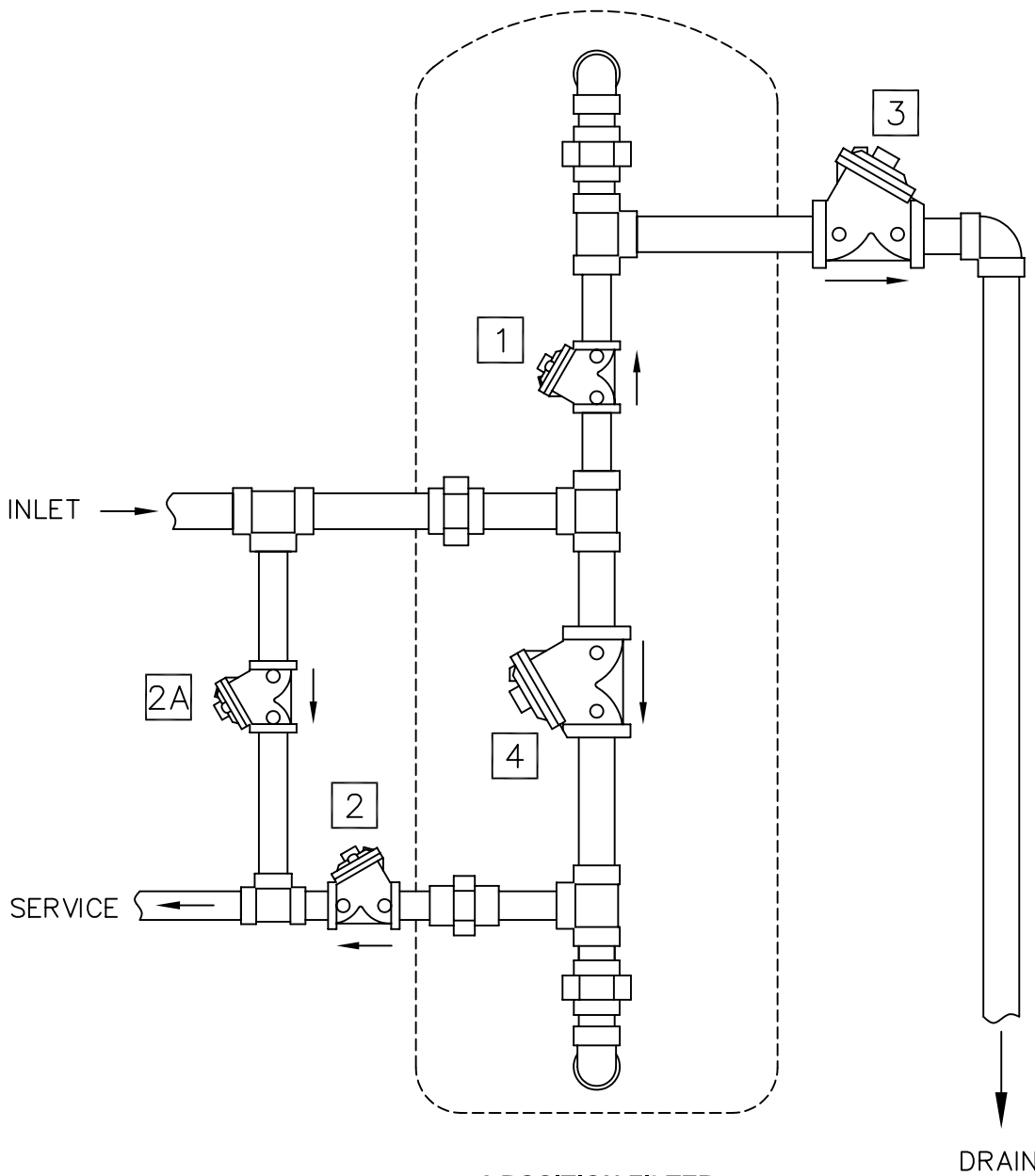
2 POSITION FILTER
